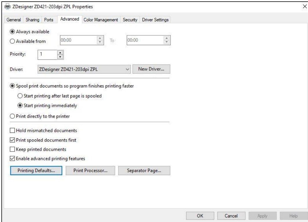
Figure 4: Printing Defaults
