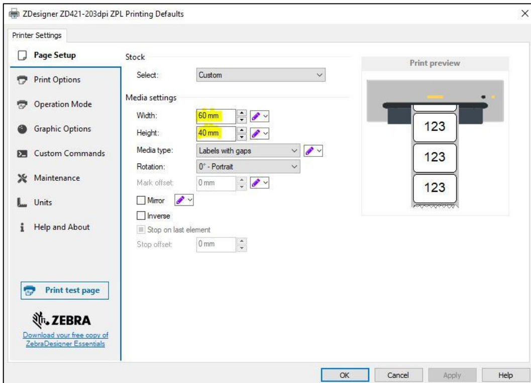
Figure 5: Page setup
